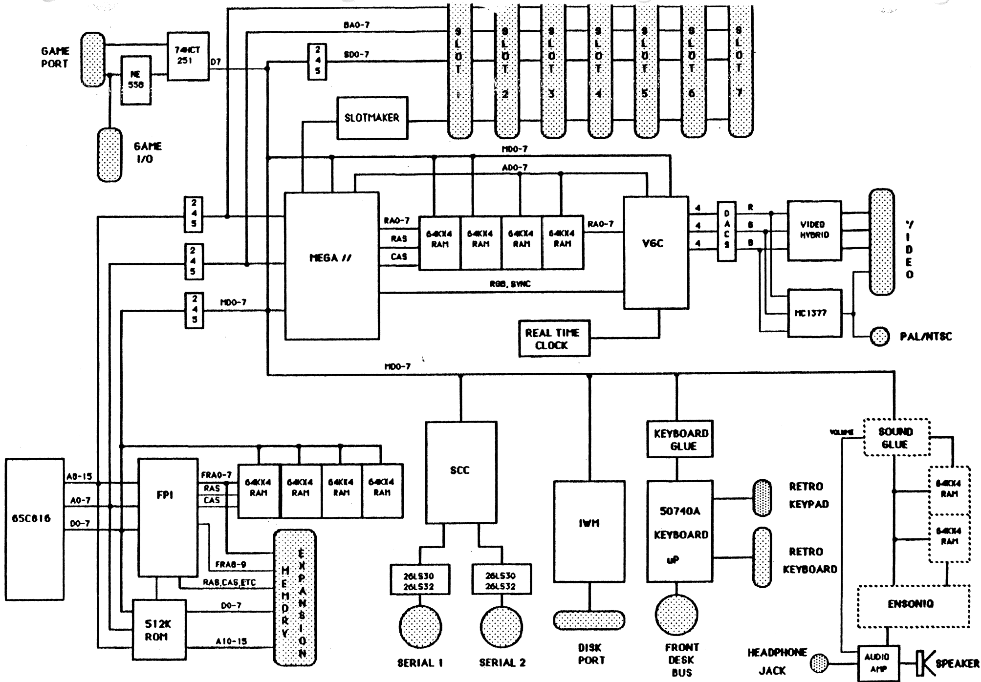
CORTLAND BLOCK DIAGRAM
